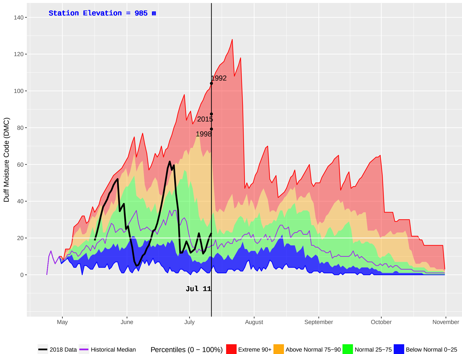
SIFTON (152) : Historical (1988–2016) and Current (2018) Noon Duff Moisture Code (DMC)
